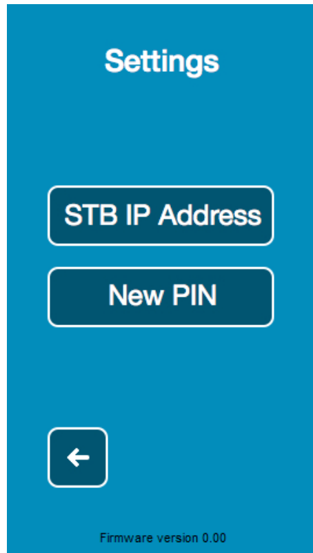
Figure 4 - Settings menu
